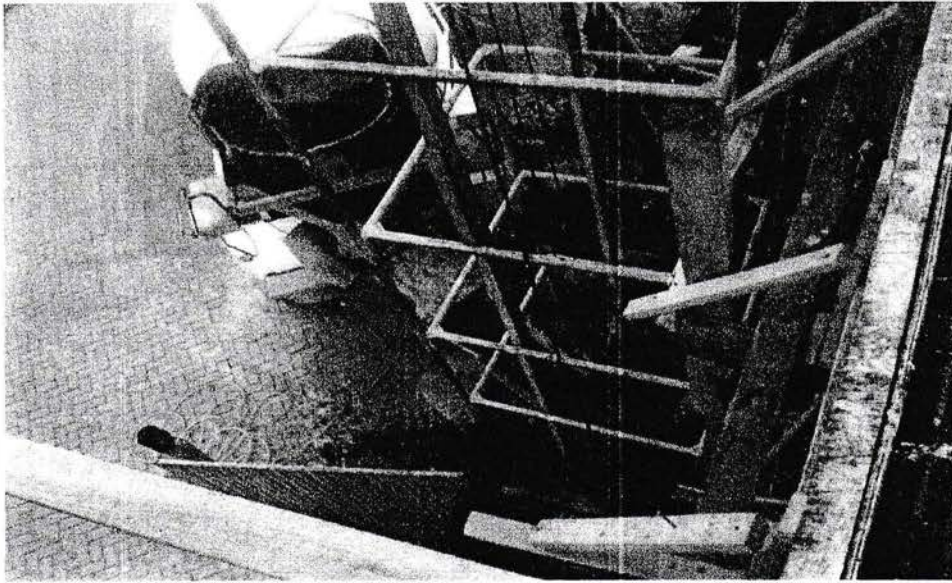
Gambar 2.10.1 Lift beton
