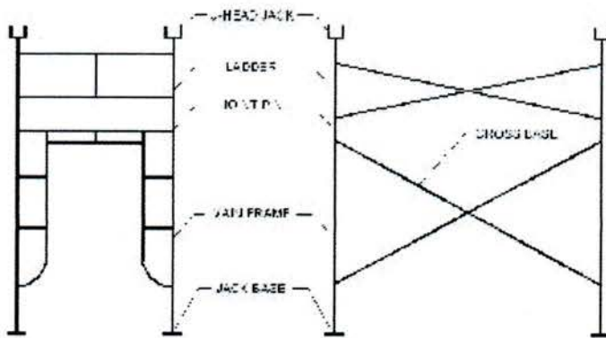
Gambar 2.9.12 Sketsa scaffolding
