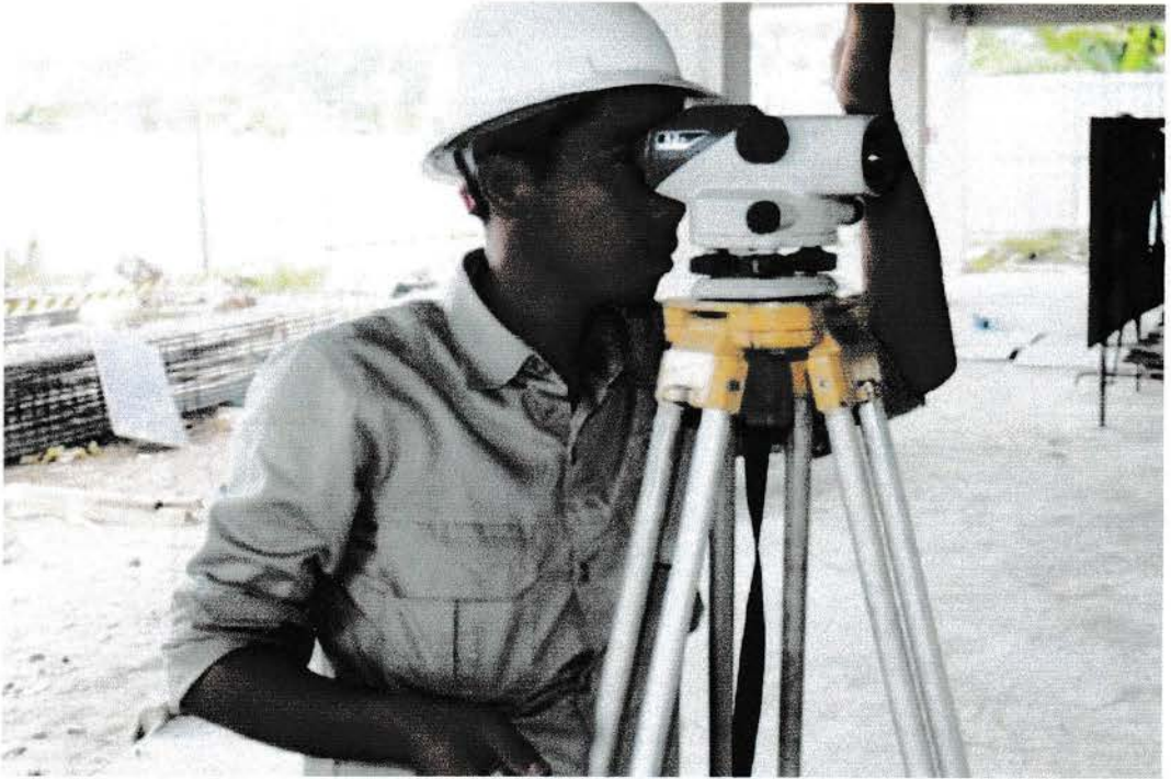
Gambar 2.9.11 Waterpass
