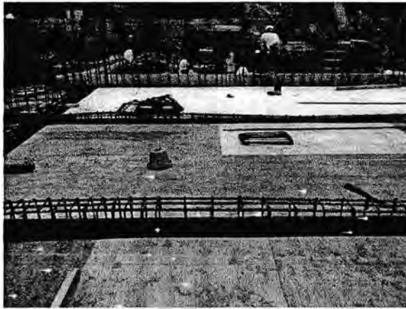
Gambar 3.16 Bekisting plat lantai
