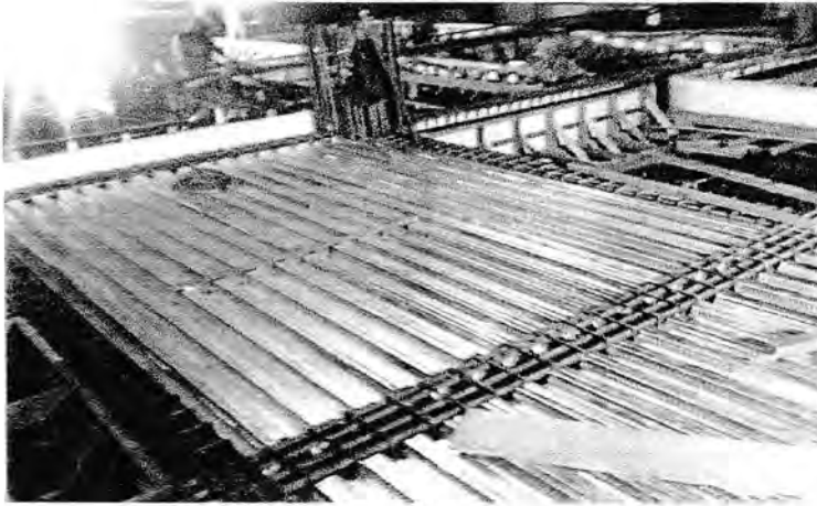
Gambar 3.3. Bekisting plat lantai
