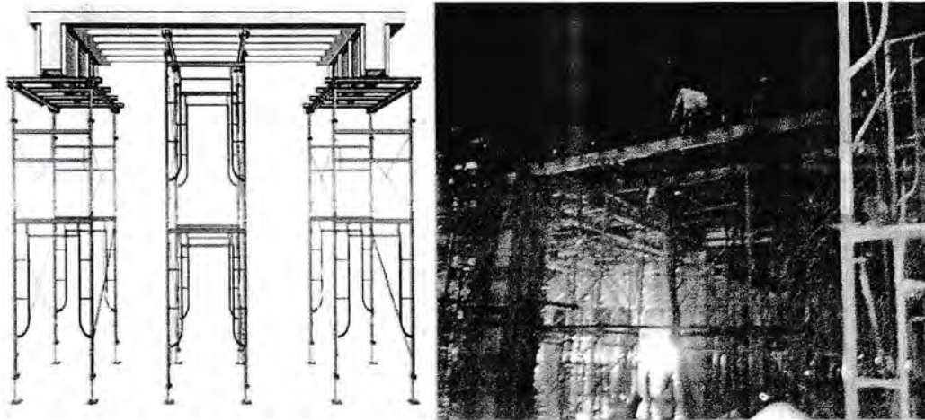
Gambar 3.2. Bekisting balok
