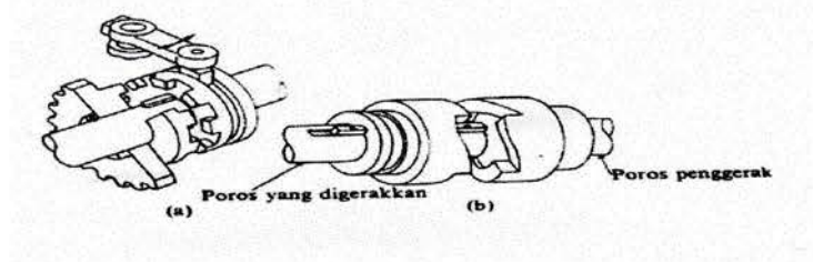
Gbr.2.9. Kopling Cakar
