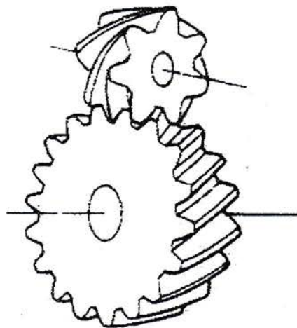
Gambar 2.7. Roda gigi miring silang.
