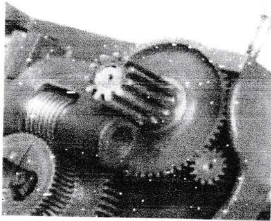
Gambar 2.8.Roda Gigi Cacing Globoid
