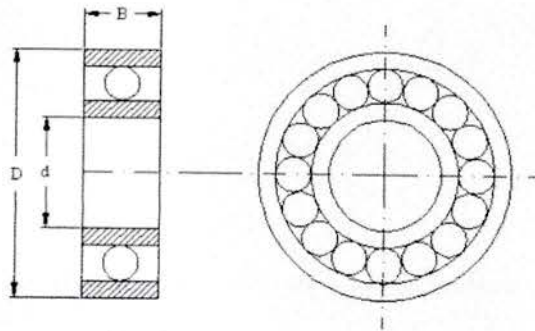
Gambar 2.16 Bantalan
