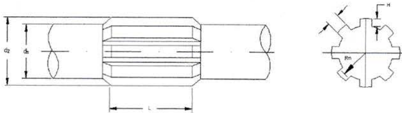
Gambar 2.14 Spline
