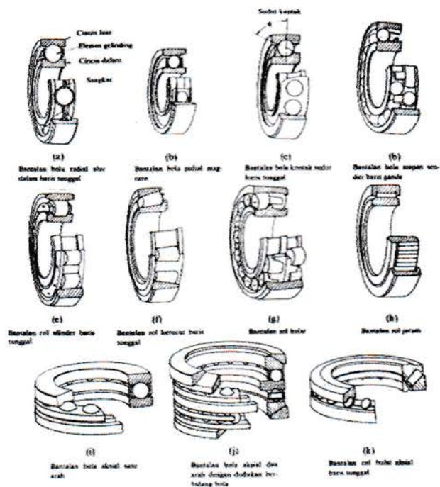
Gambar 3.5. Bantalan Gelinding
