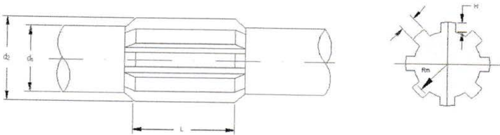
Gambar. 3.2. Spline
