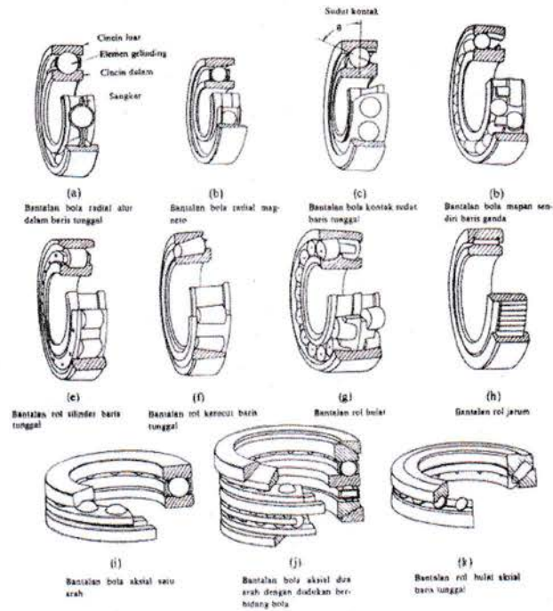
Gambar 3.5. Bantalan Gelinding
