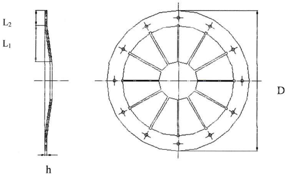
Gambar 8. 1. Pegas Matahari
