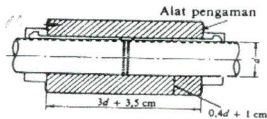
Gambar 2.1. Kopling Bus
