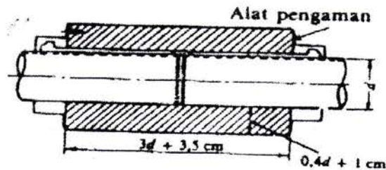
Gambar 2.1. Kopling Bus
