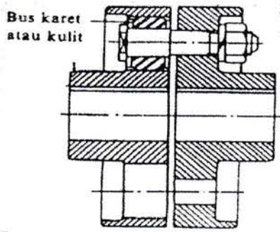
Gambar 2. 4. Kopling Flens Luwes
