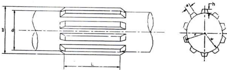
Gambar 4.1. Spline
