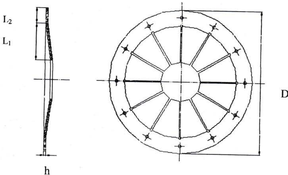
Gambar 8. 1. Pegas Matahari
