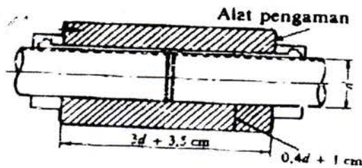
Gambar 2.1. Kopling Bus
