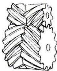
Roda Gigi Miring Ganda
