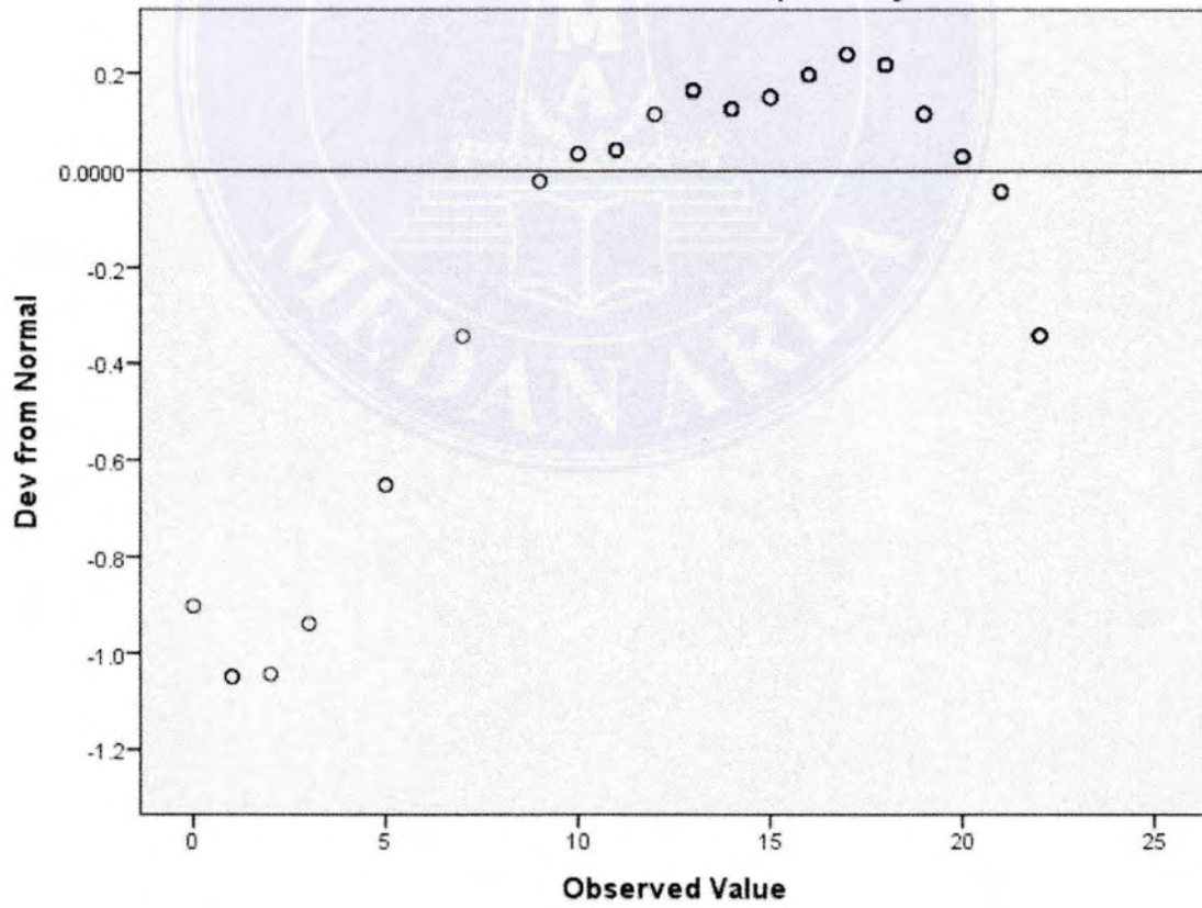
Detrended Normal Q-Q Plot of disiplinbelajar
