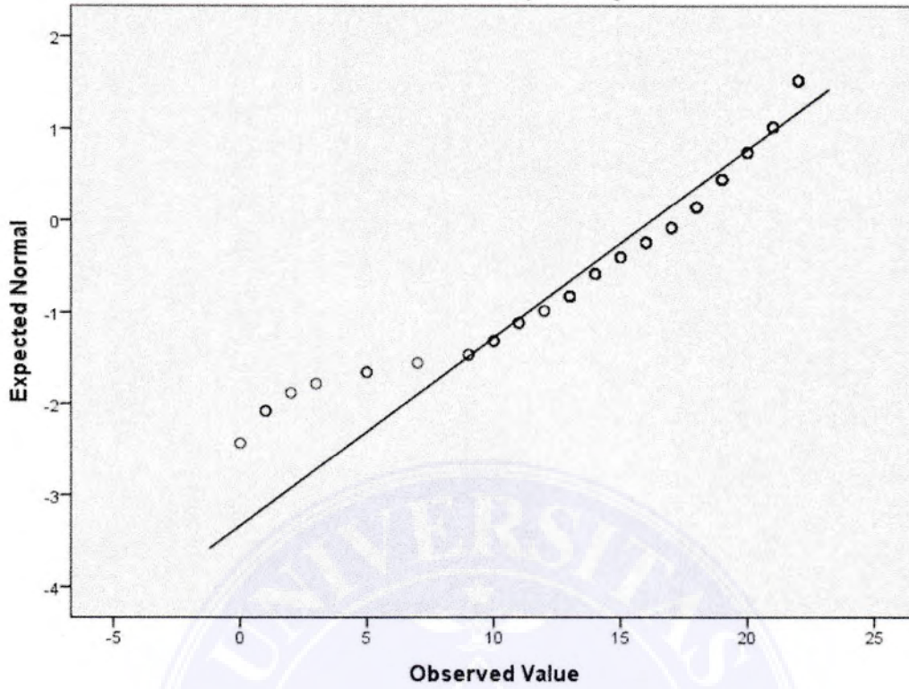
Normal Q-Q Plot of disiplinbelajar
