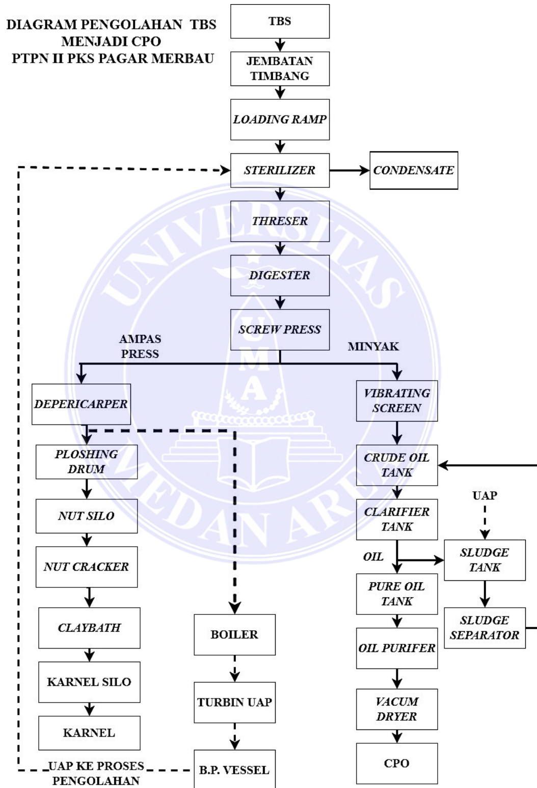
Gambar 3. 61. Blok Diagram
