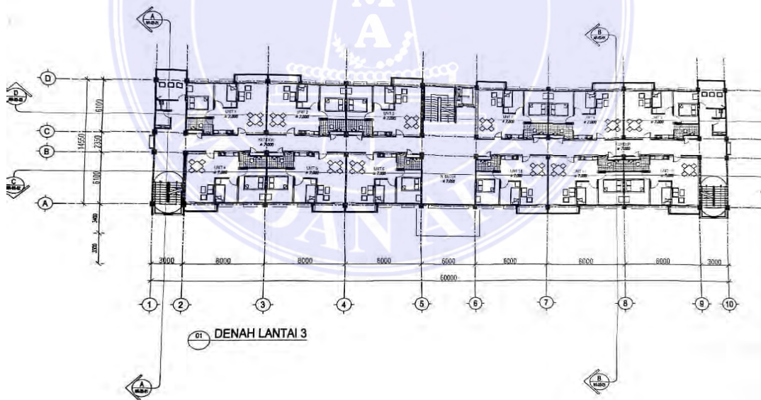
Gambar 3. Denah Lantai 3
