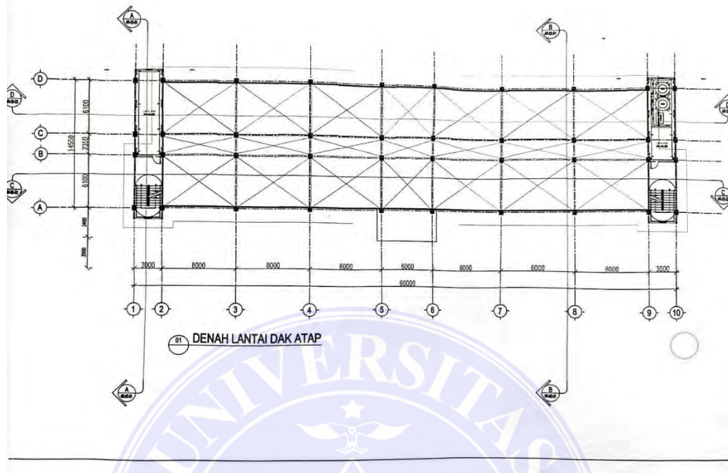
Gambar 4. Denah Lantai 4
