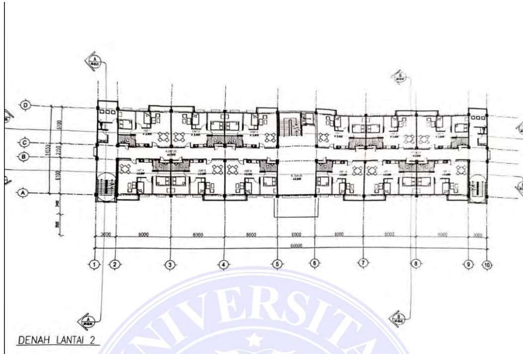
Gambar 2. Denah Lantai 2
