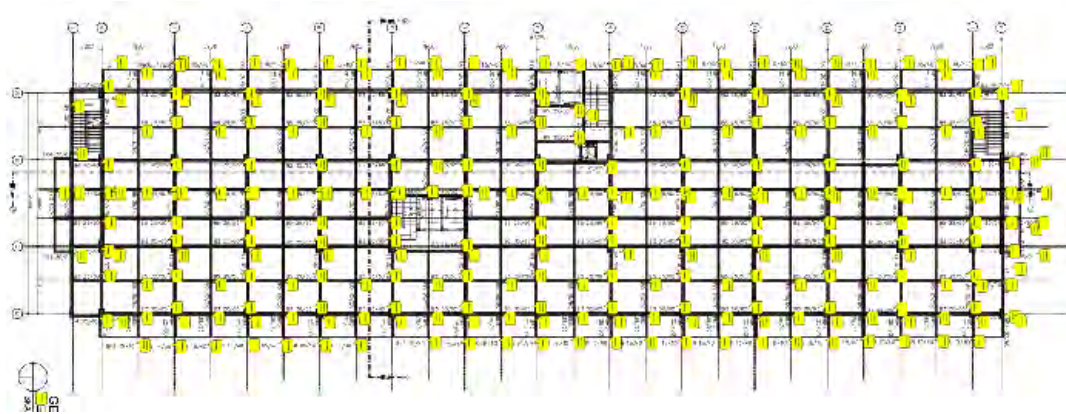
Gambar 4.2 Denah Balok
