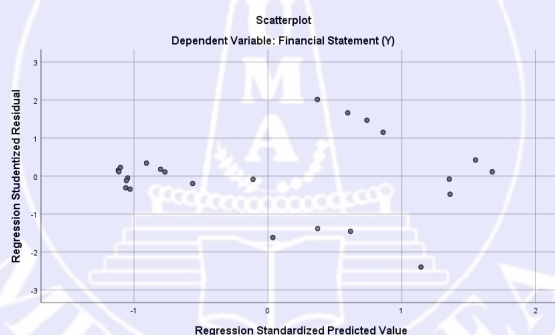
Gambar 3 Scatterplot
