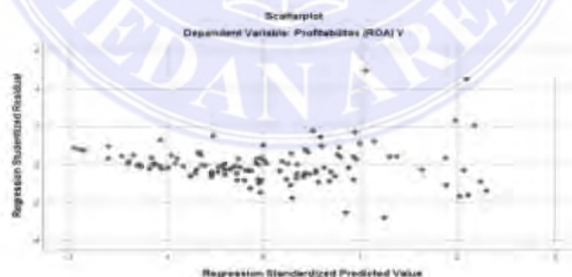
Gambar 1 Scatterplot
