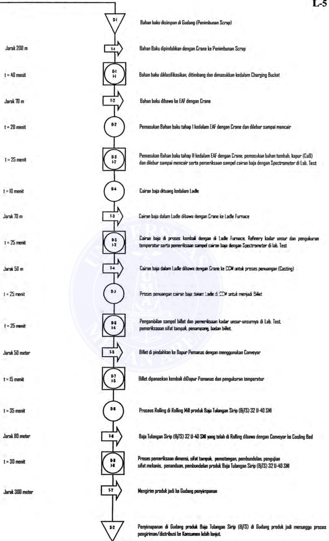
Diagram Alir Proses Produksi Baja Tulangan Sirip (BjTS) 32 U-40 SNI di PT. GROWTH SUMATRA INDUSTRY
