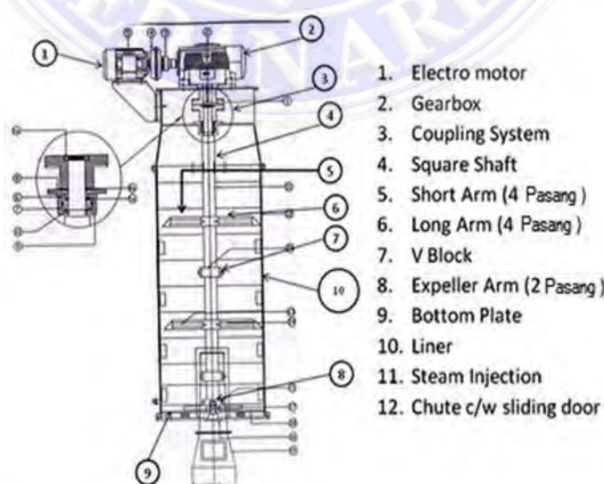
Gambar 3. 14. Bagian-Bagian Digester
