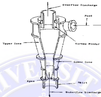
Gambar 3. 38. Bagian-Bagian Hydrocyclone
