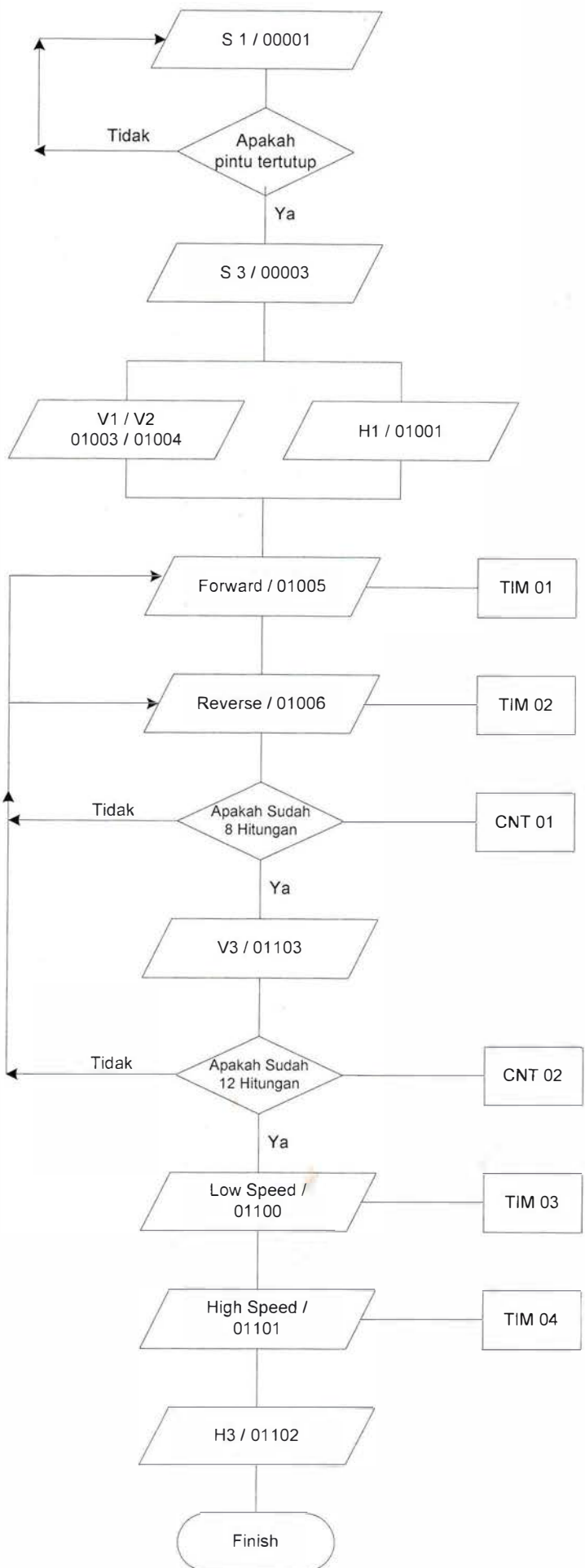
Flow Chart Proses kerja Washing Machine
