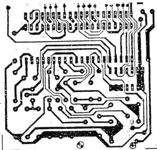
LAY OUT PCB
